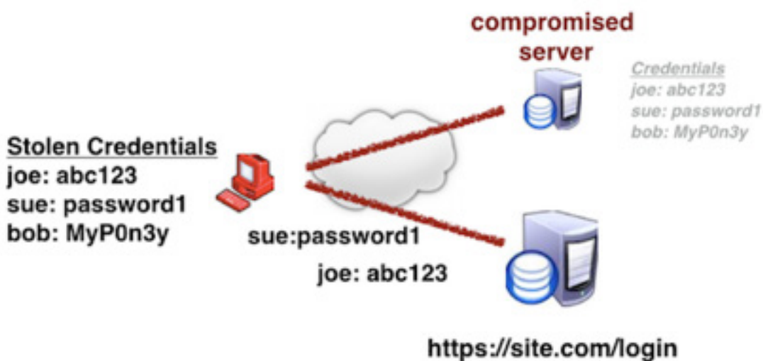
Figure 3: Credential Stuffing attack diagram by OWASP. 3
